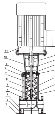
MODEL: LVR120 (150,200)
